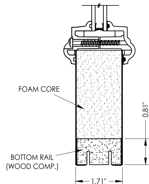
2 VERTICAL CROSS SECTION 4
