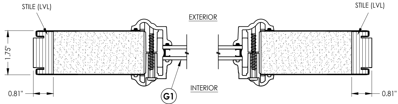
1 HORIZONTAL CROSS SECTION 4
